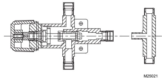
Fig. 1. UMV-304U with 4 port adapter.
